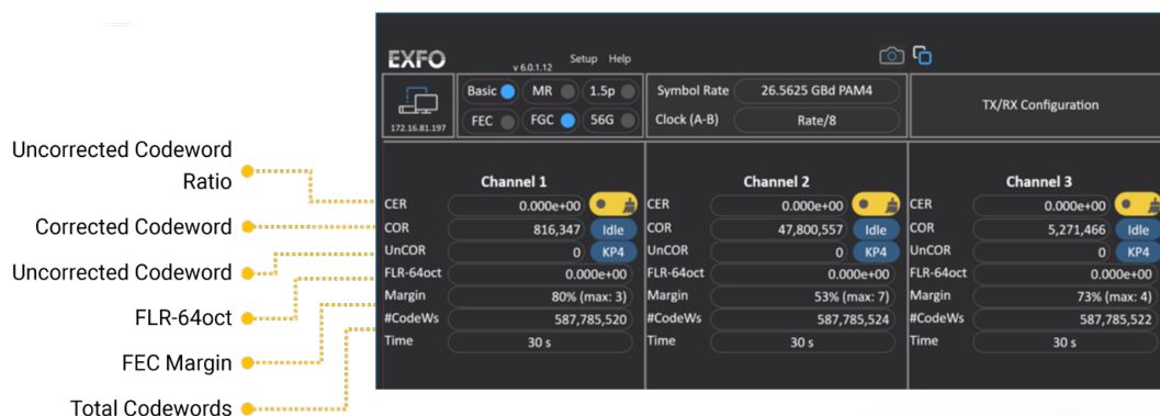
图2: BA-4000 GUI中显示的FEC Encoded Scrambled Idle码型
