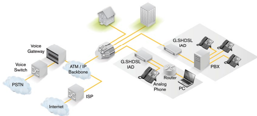
Figure 9. SHDSL architecture
