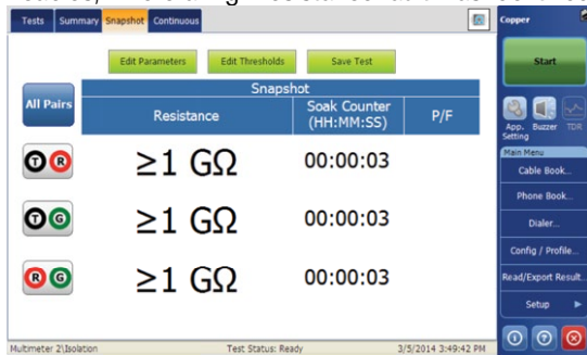
Figure 39. Isolation test
