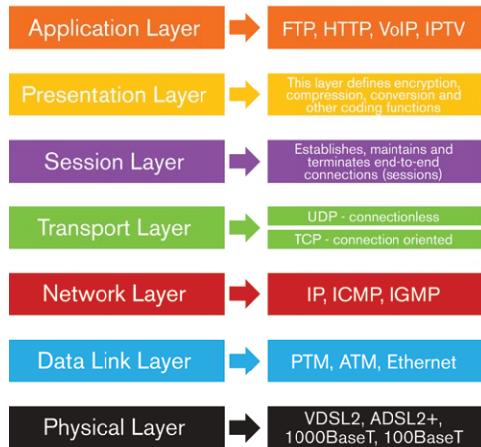
Figure 44. OSI Model
