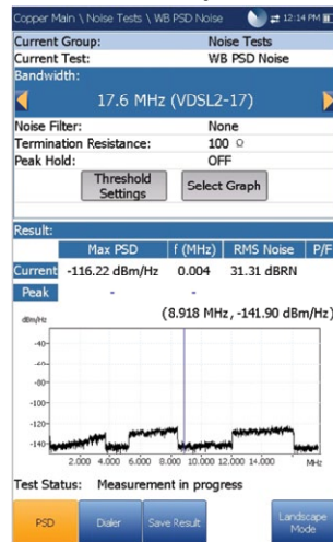
Figure 40. PSD noise test
